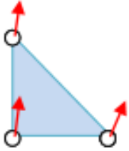
Vector data
